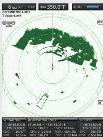
Simplified ARPA
